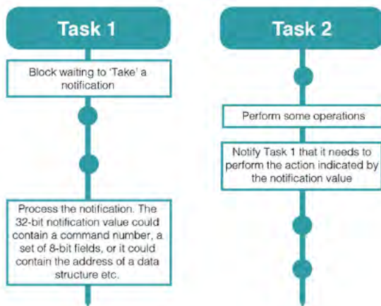
Figure 5. Using Task Notifications as a lightweight mailbox
