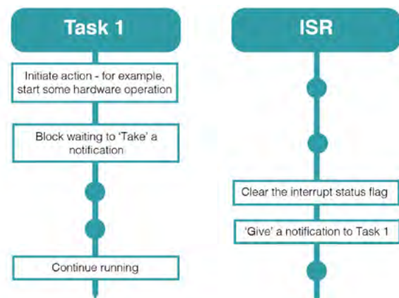
Figure 2. Using Task Notifications as a binary semaphore between an ISR & a task
