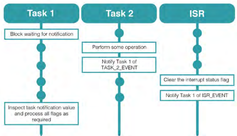
Figure 4. Using Task Notifications as an Event Group
